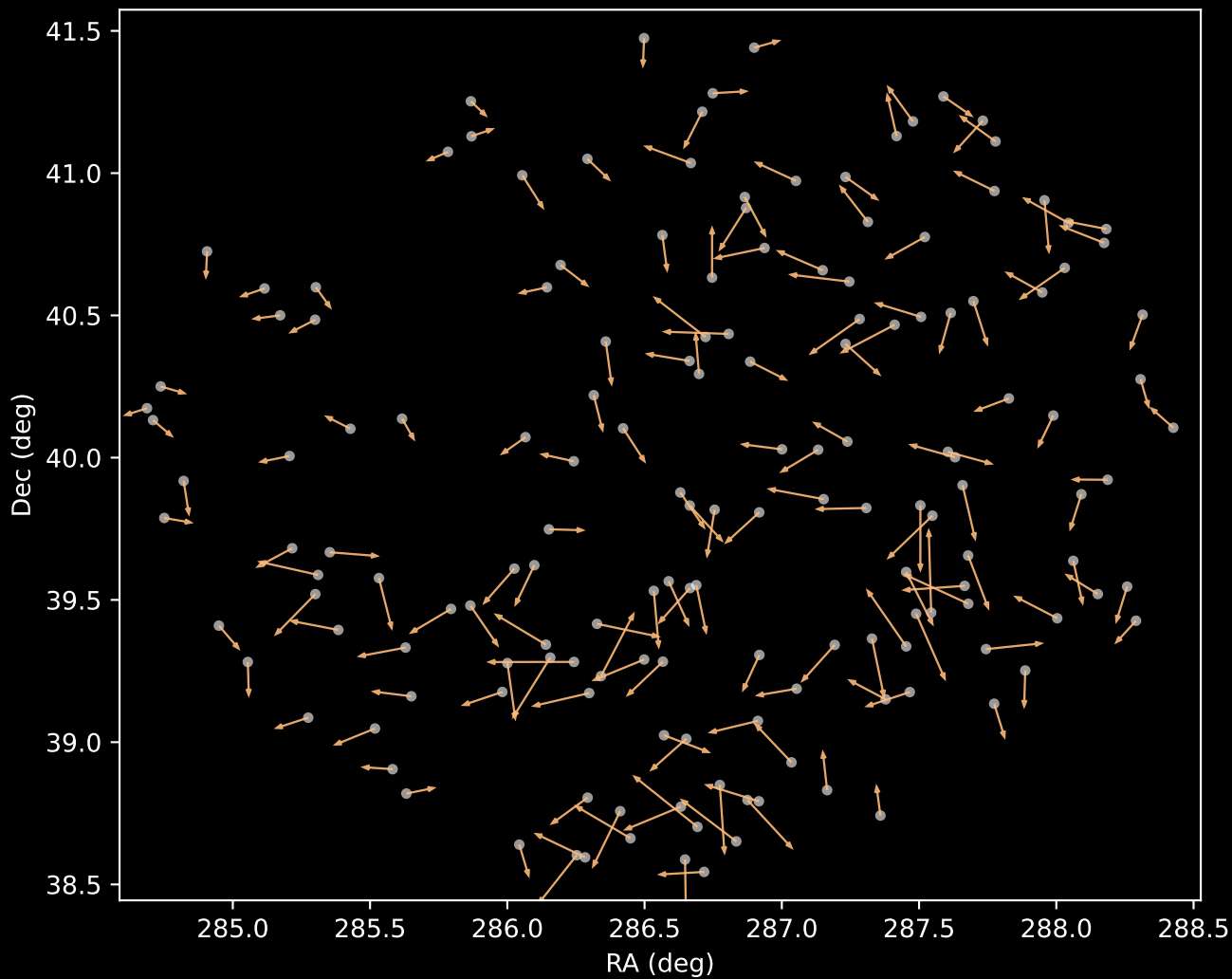
APOGEE DR17 Cluster 3 Proper Motion Vectors (n=159)
