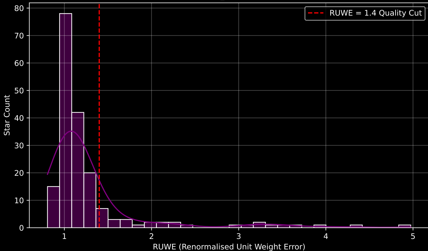
GAPOGEE DR17 Field [143+76_MGA] RUWE Distribution (n= 186)
