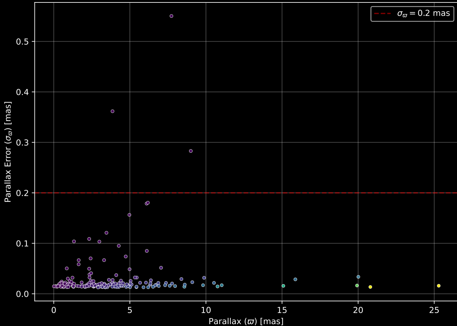
APOGEE DR17 Field: [143+76_MGA] Parallax Quality (n= 197)
