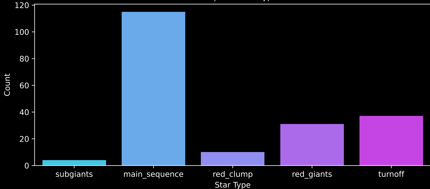
APOGEE DR17 Field: [143+76_MGA] Count plot of Star Type
