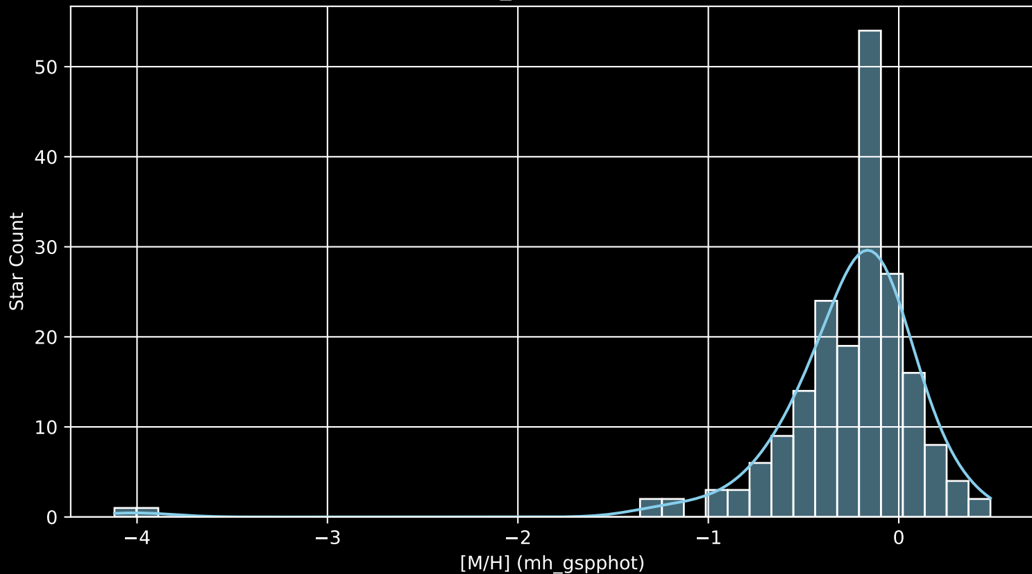
APOGEE DR17 Field: [143+76_MGA [M/H] (mh_gspphot) (n= 195)
