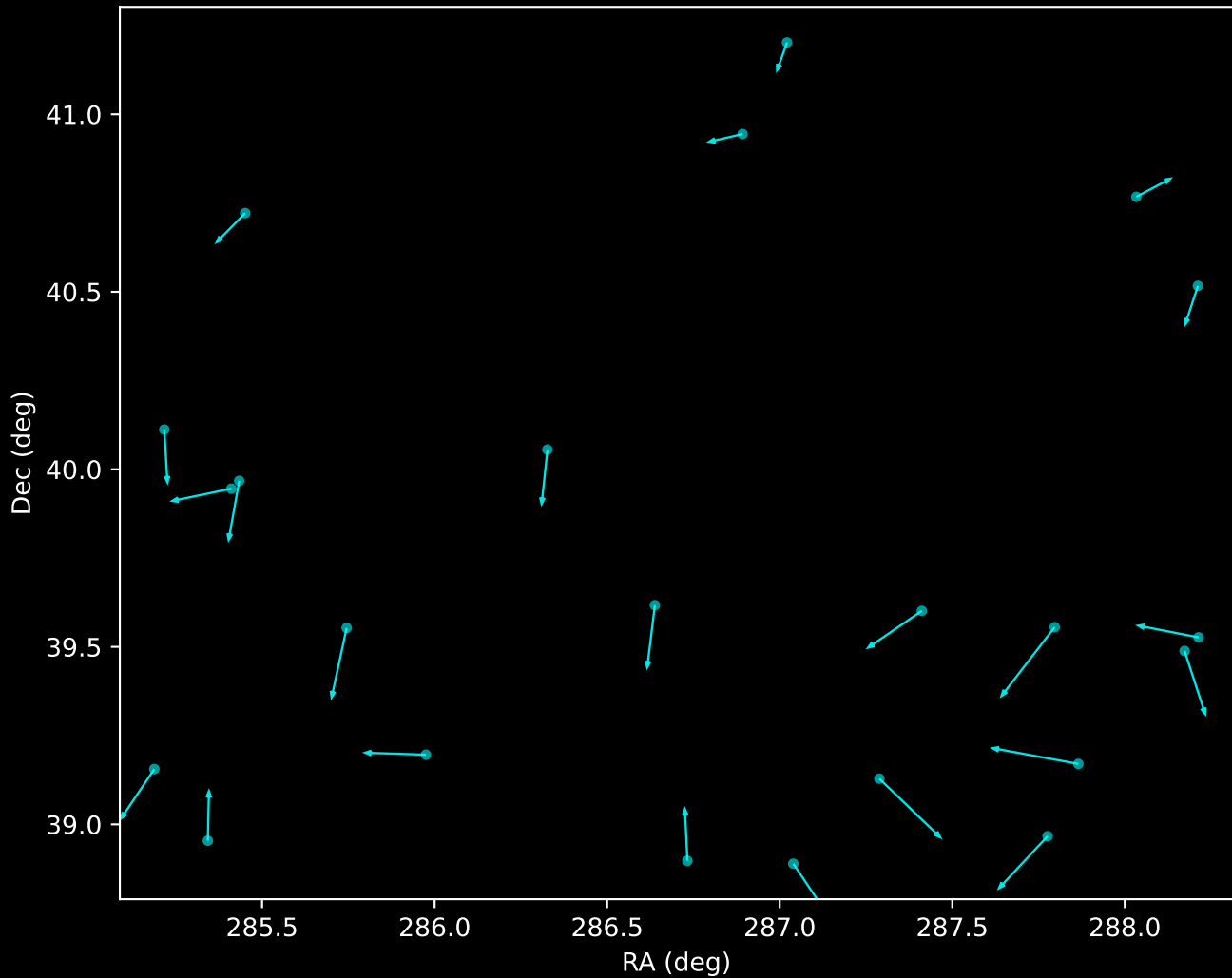
APOGEE DR17 Noise Stream Proper Motion Vectors (n=23)
