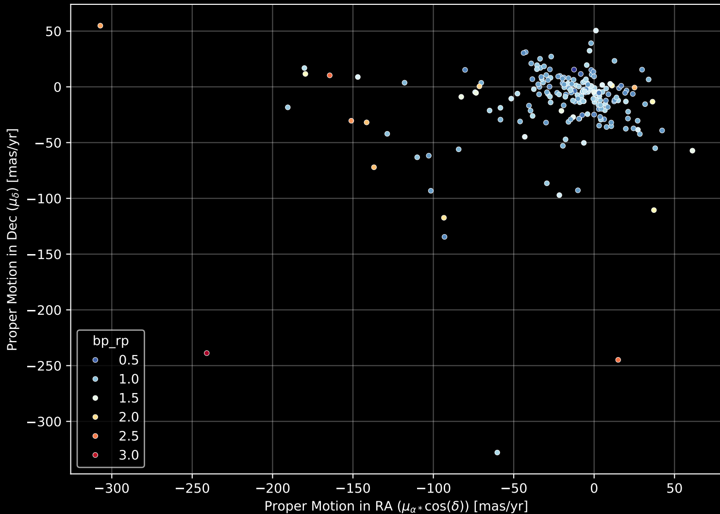
APOGEE DR17 Field: [143+76_MGA] Proper Motion Diagram (n= 197)
